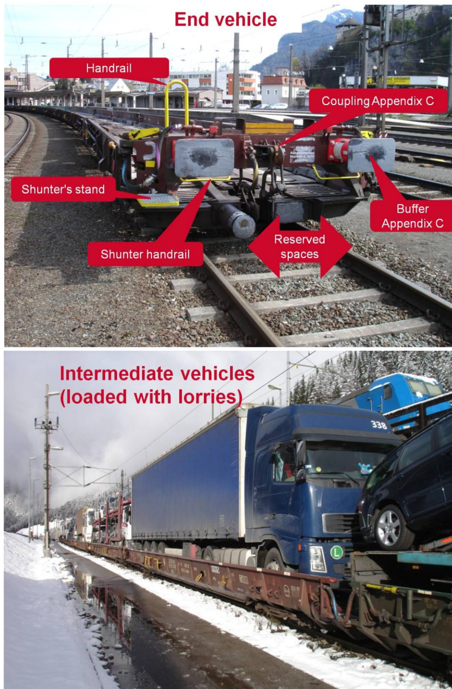
Figure 9: Example of a unit to carry lorries (“Rollende Landstrasse”)
