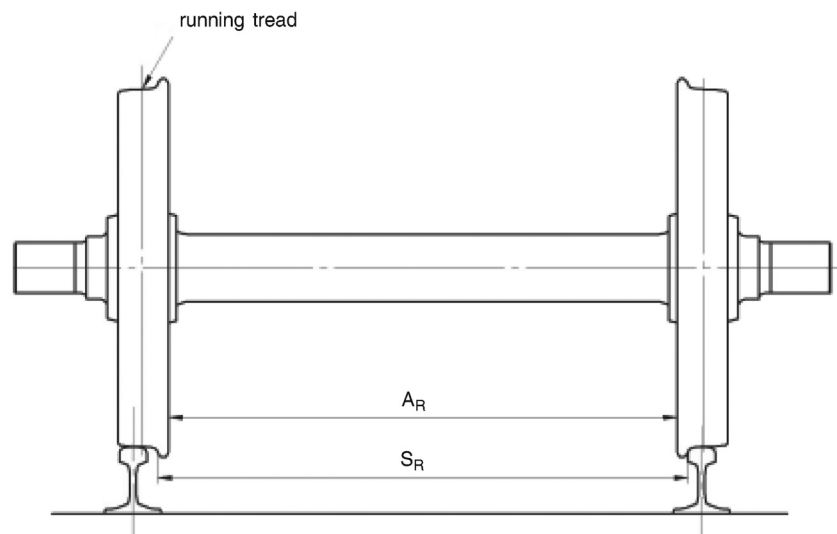
Symbols for wheelsets used in Table 3
