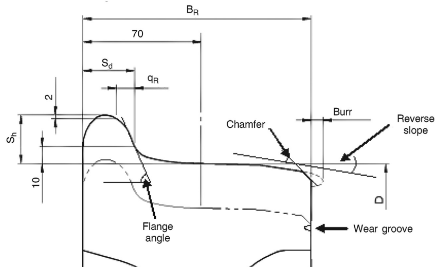
Symbols for wheels used in Table 4
