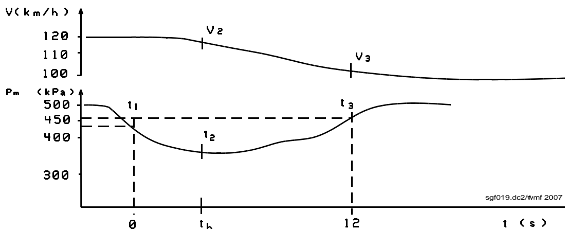
Figure 5.7-1. Deceleration measurement
