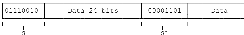
Figure 5.4-1. Synchronization words in a balise telegram
