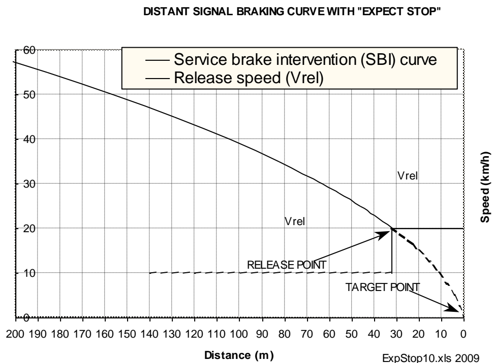
Figure 4.6-1. Note. Release point for an Expect Stop distant signal braking
