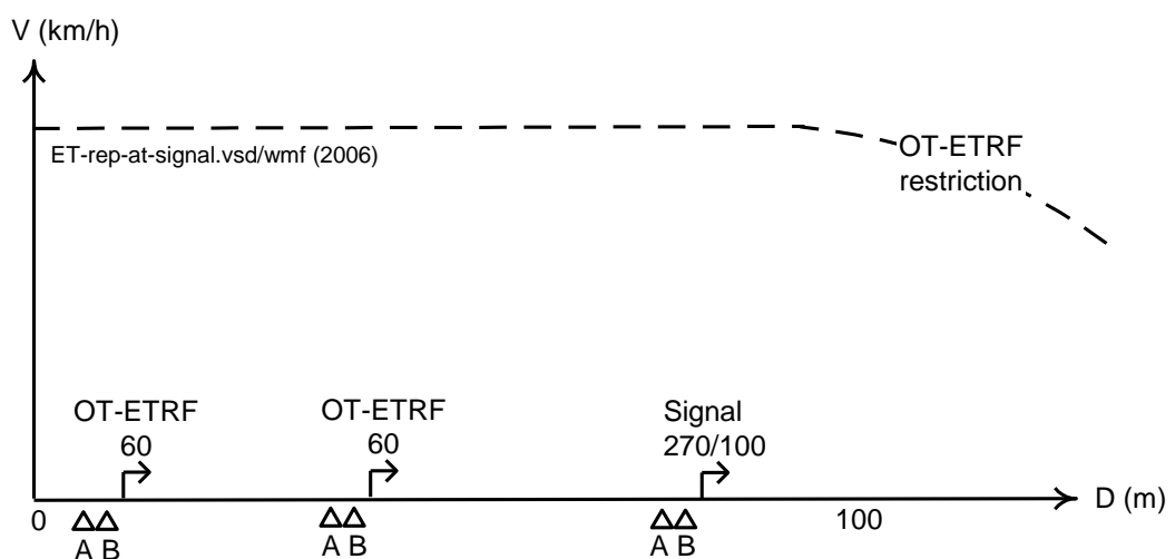
Figure 4.4-1. Repetition of OT-ET at the same signal
