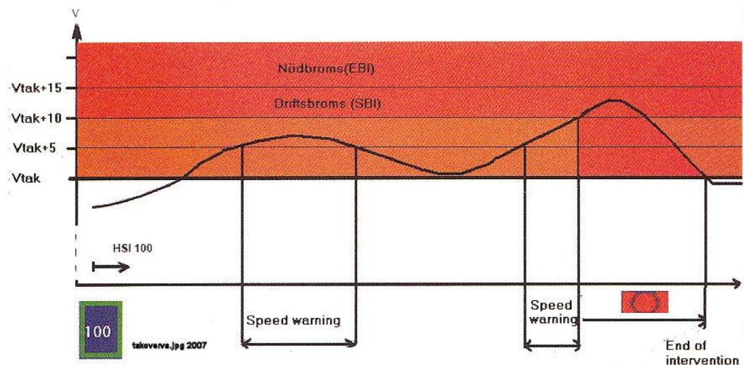
Figure 4.5-1. Max speed supervision with MARGIN BAR colours
