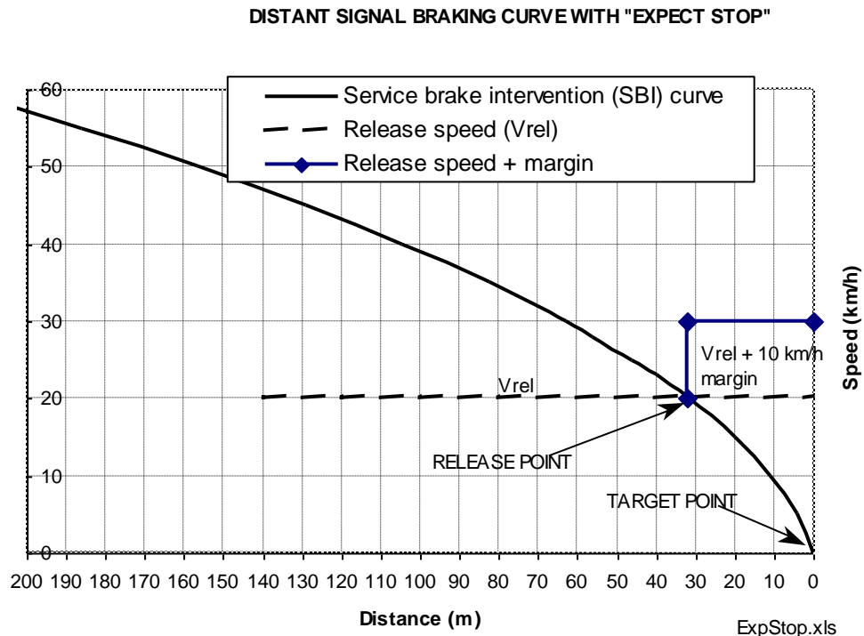
A-Figure 4.6-2. A-note. Release point for an Expect Stop distant signal braking curve.
