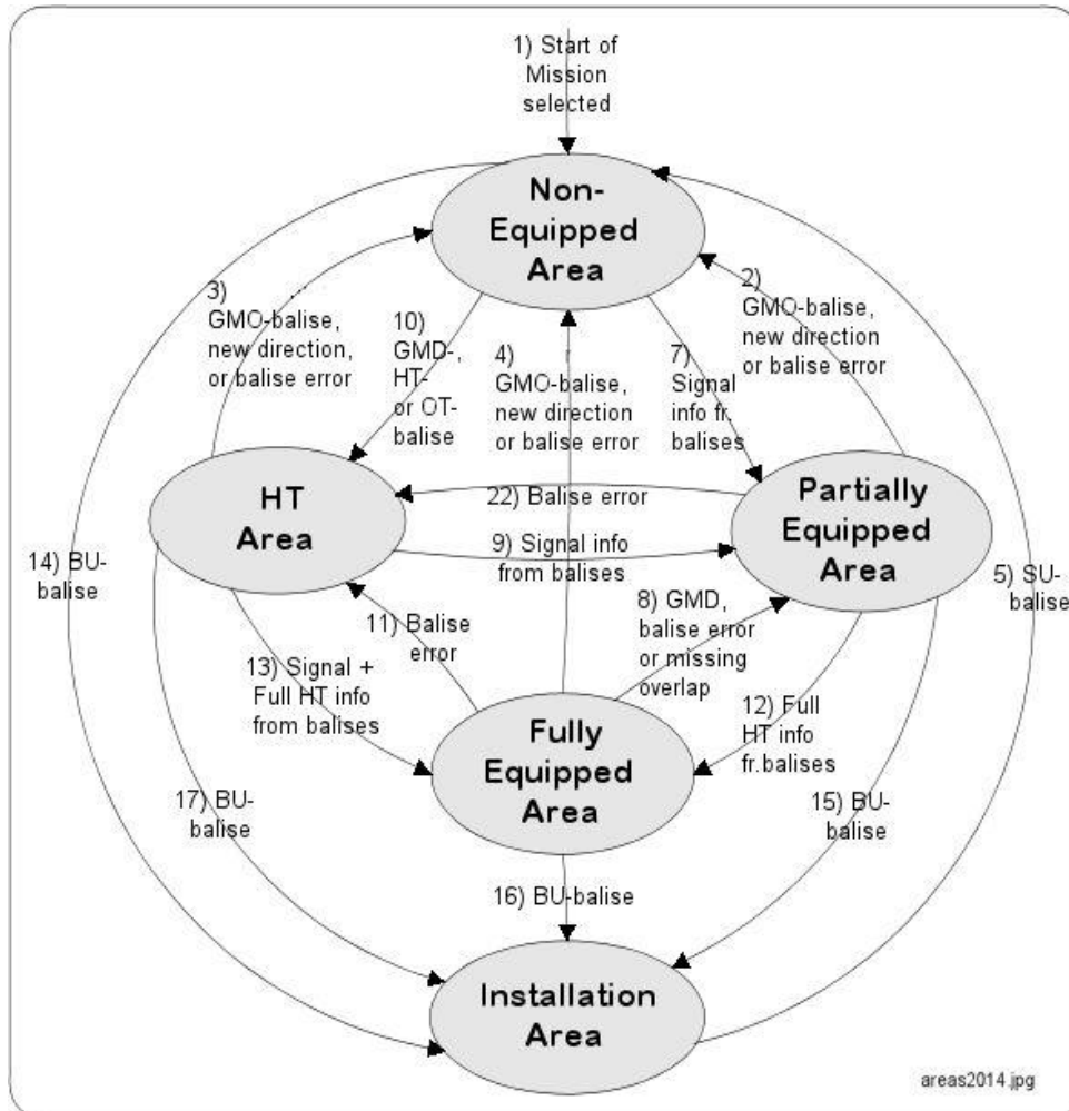
Figure 4.4-1. Area transitions
