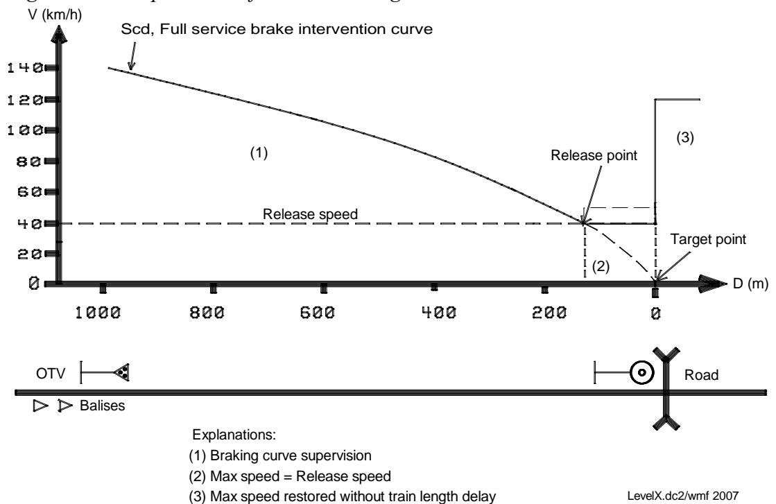
Figure 4.6-3. Supervision of a level crossing
