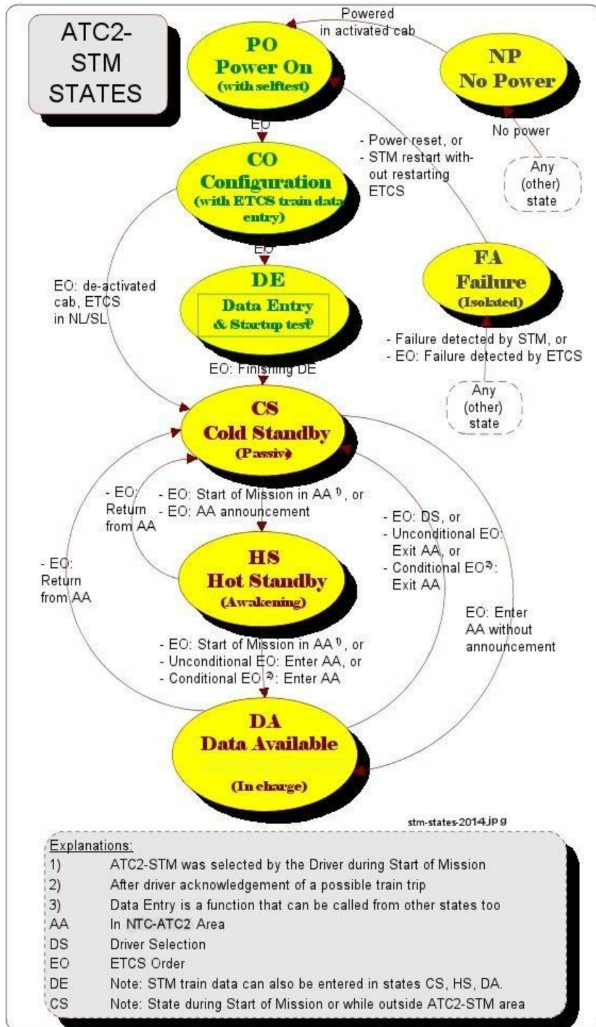
Figure 4.3-1. Note. STM State Transitions
