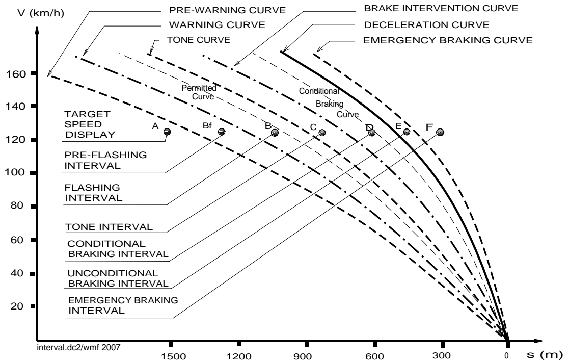
Figure 4.9-1: Summary of the various intervals
