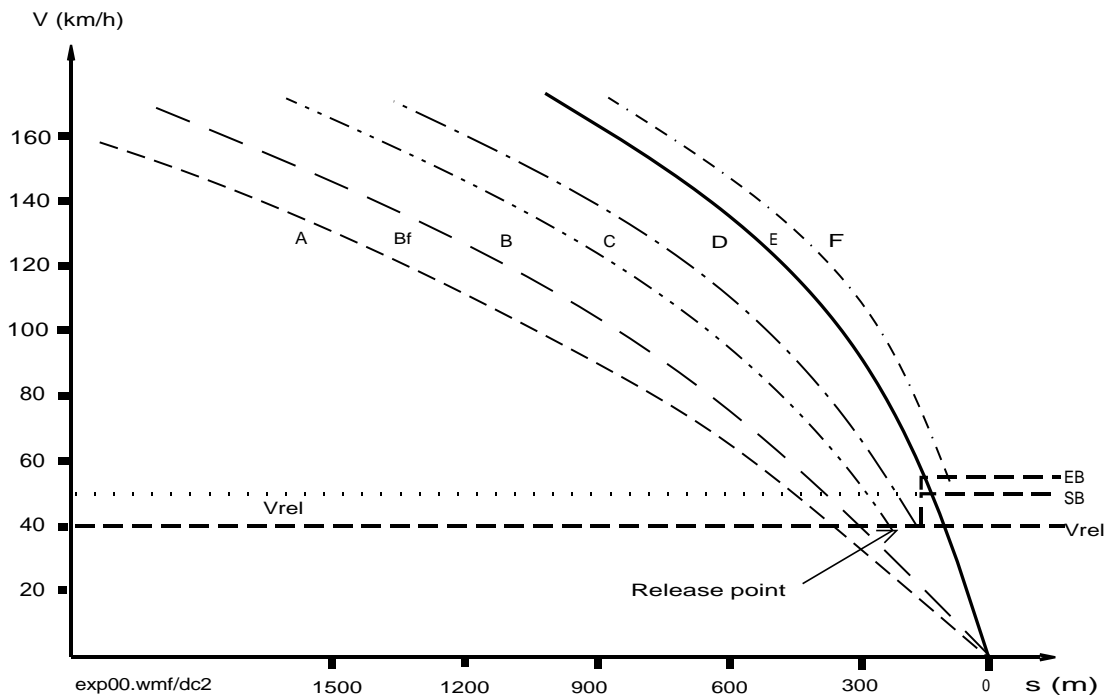
Figure 4.9-2. The position of the release point at 40-supervision
