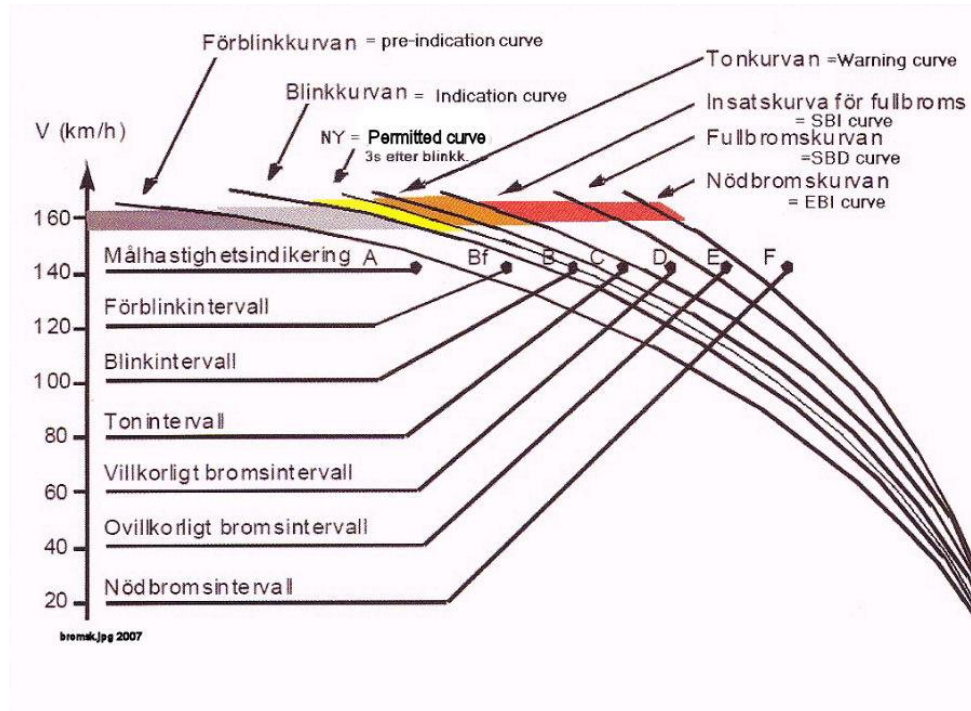
Figure 4.6-4. Braking curve intervals that affect the indications
