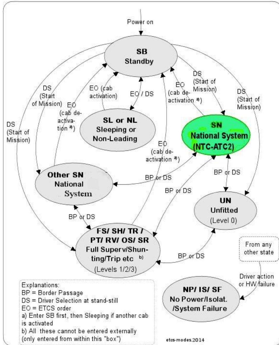
Figure 4.3-2. ETCS Mode & Level Transitions Overview
