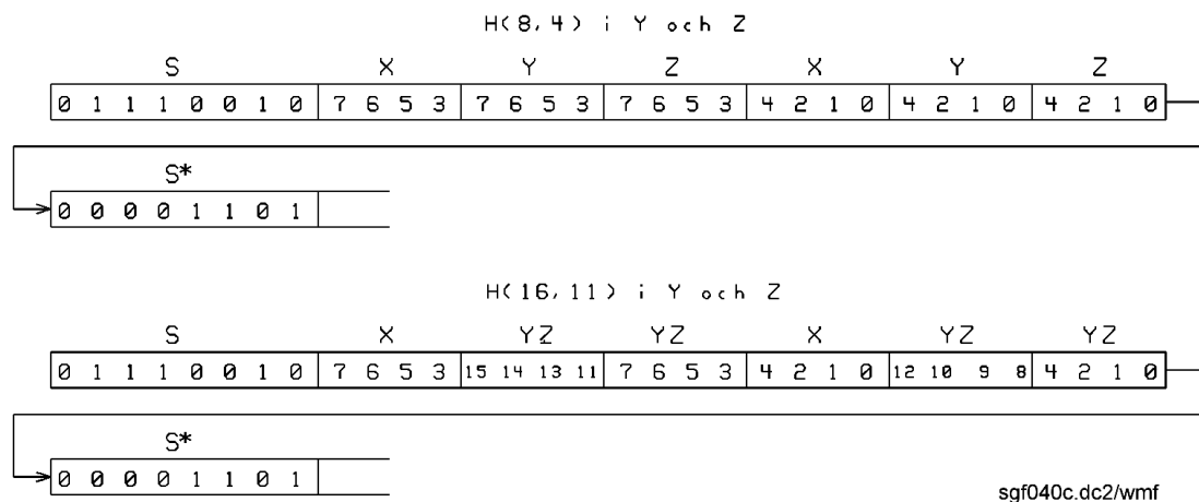
Figure 3.2-1. Telegram layout
