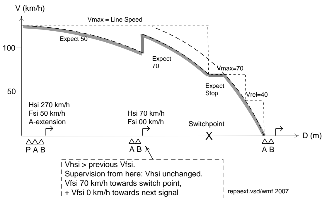
Figure 3.6-3. Passage of combined signal during category A extension
