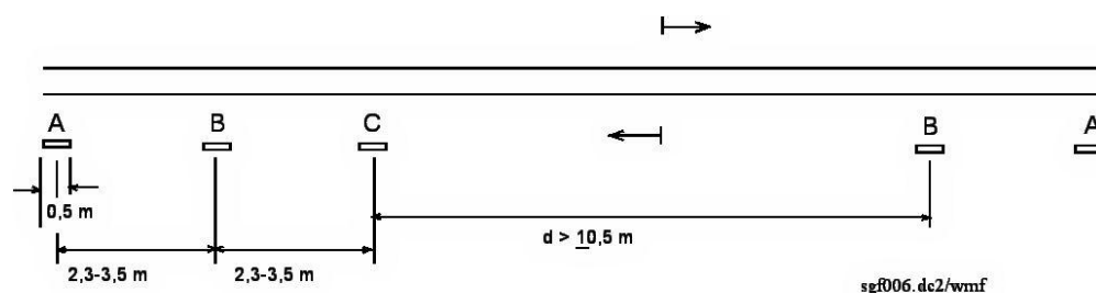
Figure 3/3-1. Distances between balises and balise groups
