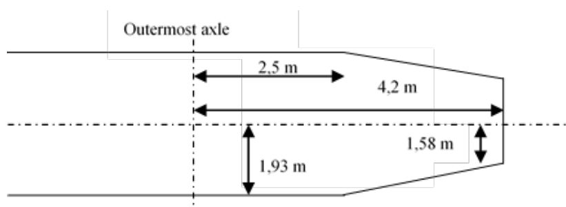
Figure 5.2 Maximum vehicle width including end-throw outside outermost axle.
