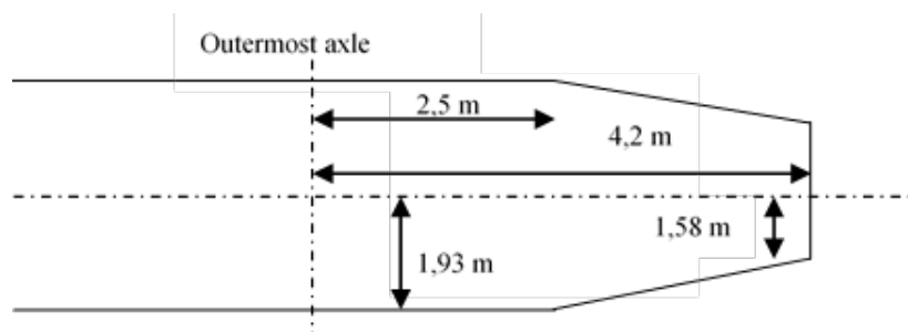
Figure 6.2 Maximum vehicle width including end-throw outside outermost axle.
