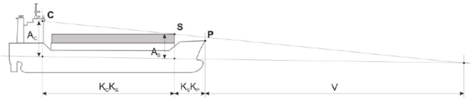
Figure 3.1. Distances used for calculating the bridge visibility
