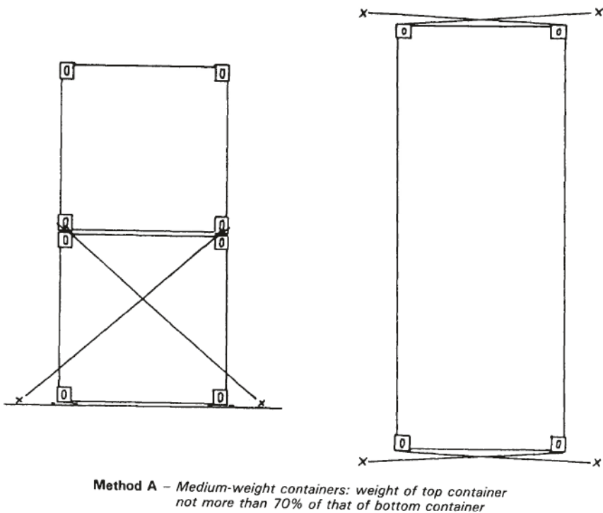
Figure 1 – Recommended methods of non-standardized securing of containers
