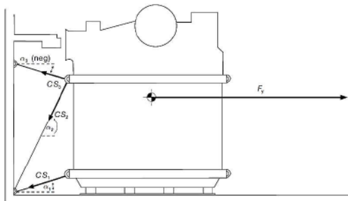
Figure 17 – Balance of transverse forces
