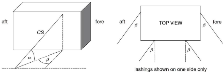
Figure 19 – Definition of the vertical and horizontal securing angles \alpha and \beta
