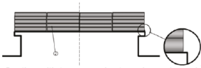
Section with transversely stowed round wood secured by friction only (Alternative 1). Non-slip paint on hatch cover or non-slip material between hatch cover and round wood should be used.
