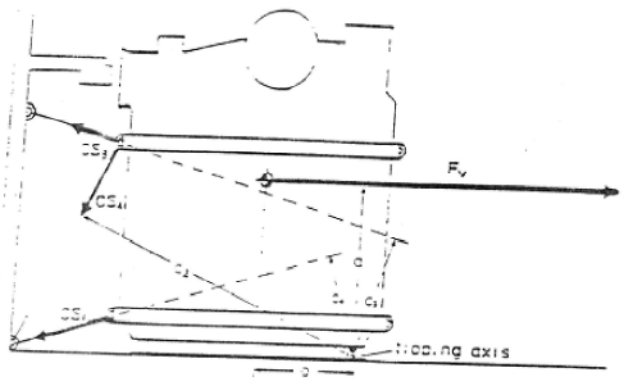
Figure 2: Balance of transverse moments
