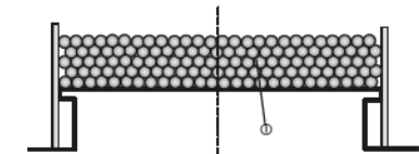
Section with longitudinally stowed round wood secured by uprights.
