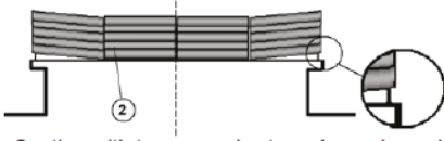
Section with transversely stowed round wood secured by friction only (Alternative 2). Non-slip paint on hatch cover or non-slip material between hatch cover and round wood should be used.
