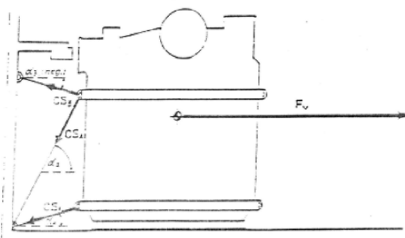
Figure 1: Balance of transverse forces
