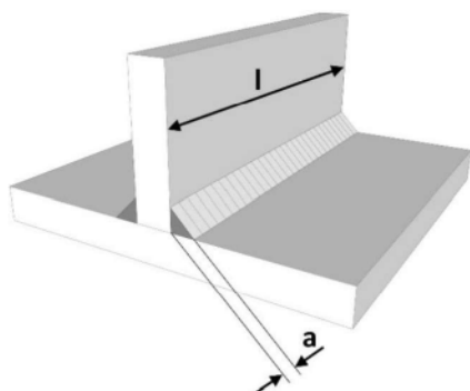
Figure 16.1 – Welding of steel stoppers
