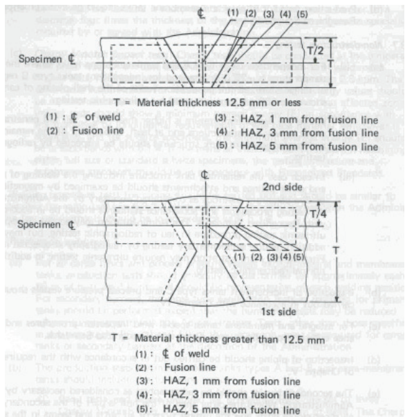
Figure 6.1 - Orientation and location of Charpy V-notch specimen
