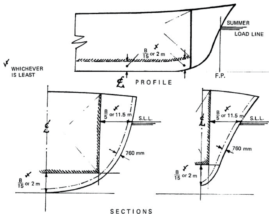
Figure 2.1 - Tank Location Requirements as set out in 2.6
