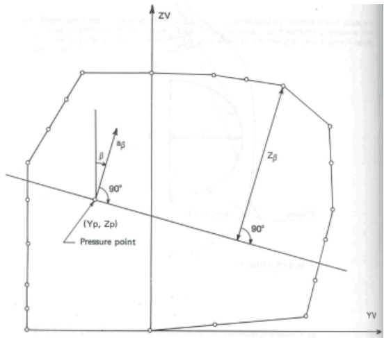
Figure 4.2 - Determination of Internal Pressure Heads
