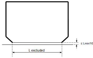
Prismatic tanks
