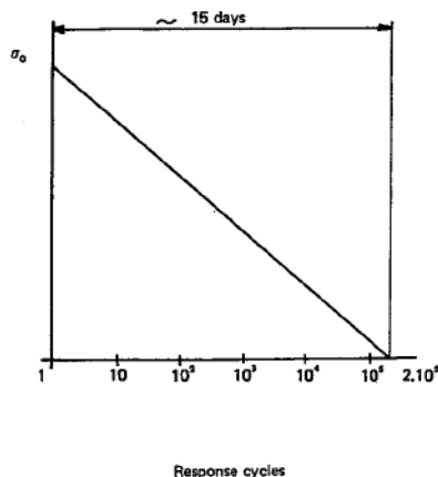
\sigma_0 = most probable maximum stress over the life of the ship Response cycle scale is logarithmic; the value of 2.10^5 is given as an example of estimate.
