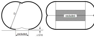
Bilobe tanks
