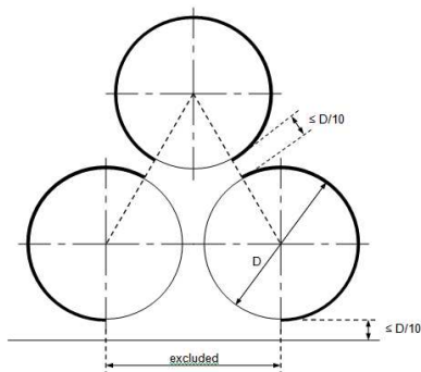
Horizontal cylindrical tanks arrangement
