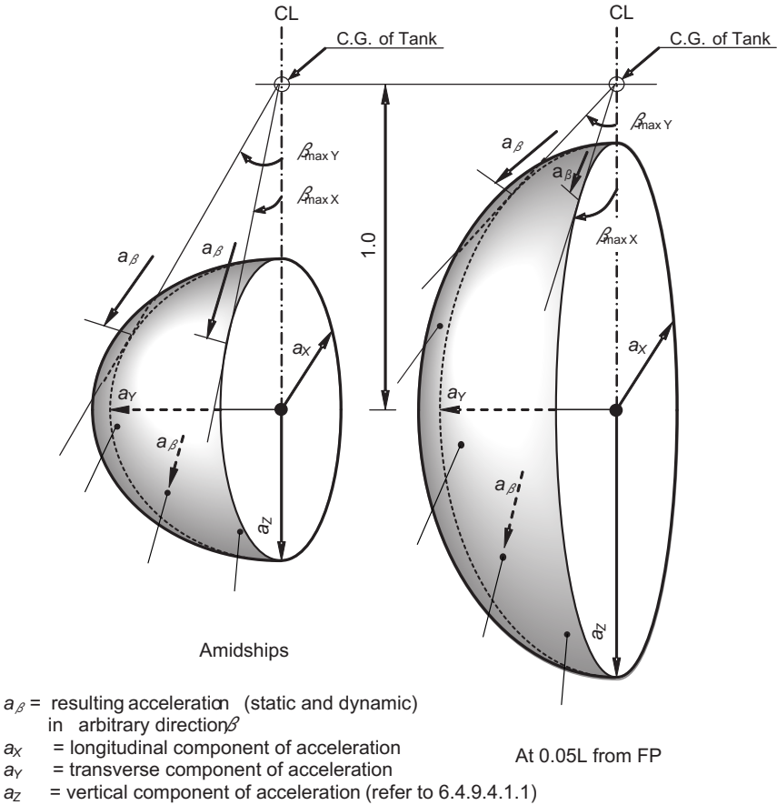
Figure 6.4.1 – Acceleration ellipsoid
