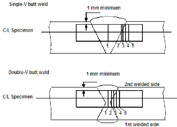
Figure 16.2 – Orientation of weld test specimen
