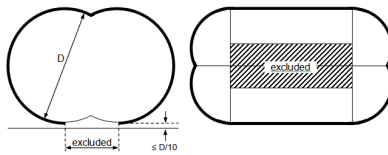
Bilobe tanks
