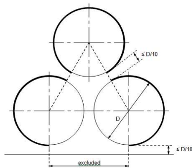
Horizontal cylindrical tanks arrangement
