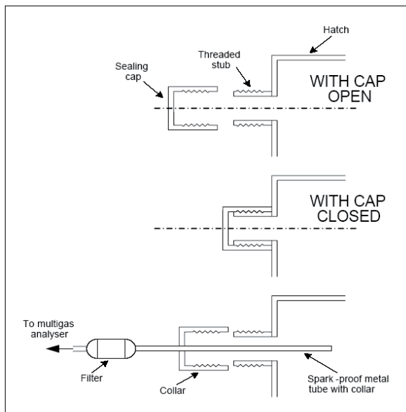
Diagram of gas sampling point
