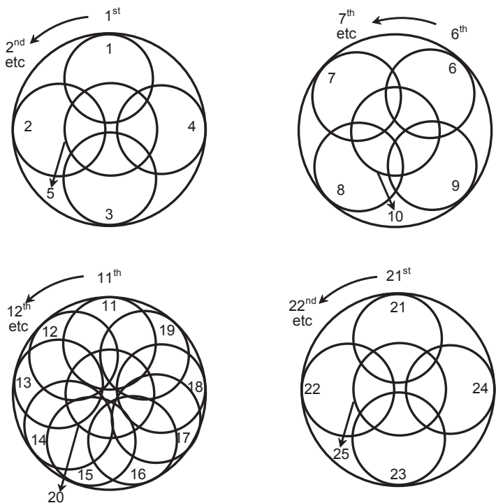
Figure 1.5.6 Recommended compaction patterns
