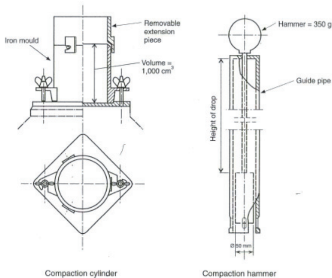
Figure 1.3.2 – Proctor apparatus
