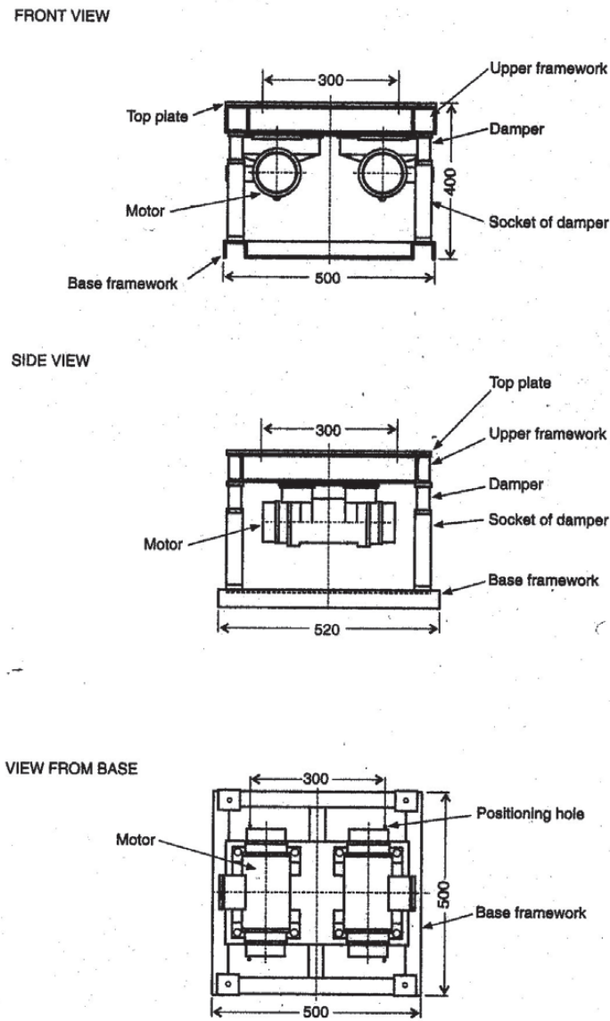
Figure 1.2.2.2 – Vibration table
